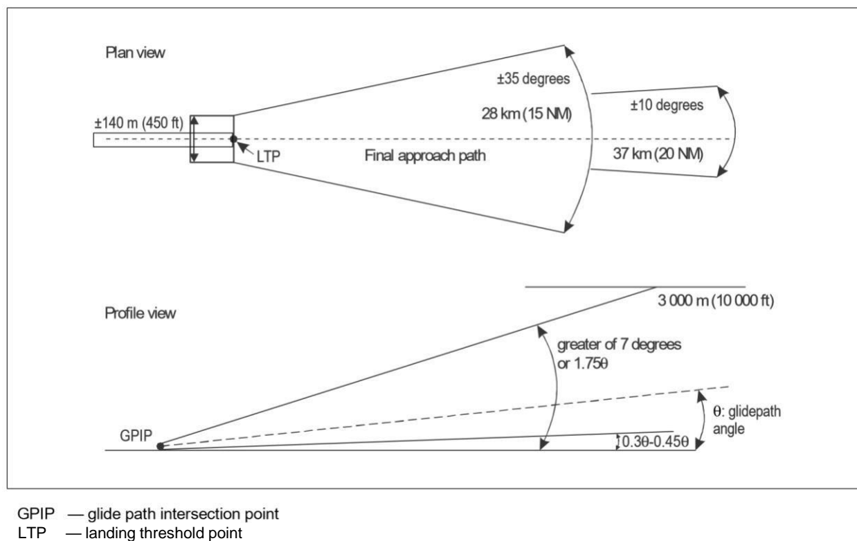
Figure D-5. Minimum GBAS service volume
