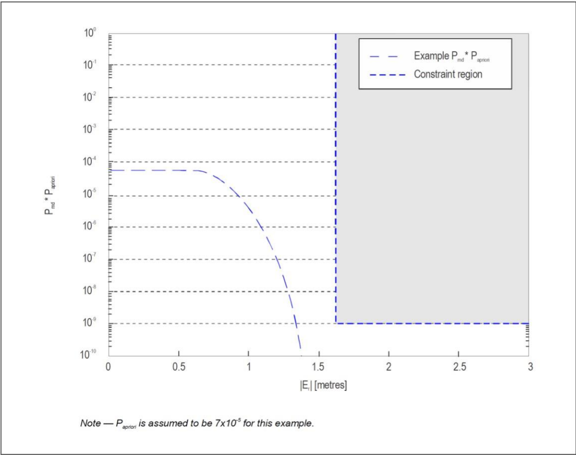
Figure D-12. Example P_{md\_limit} constraint with a priori probabil
