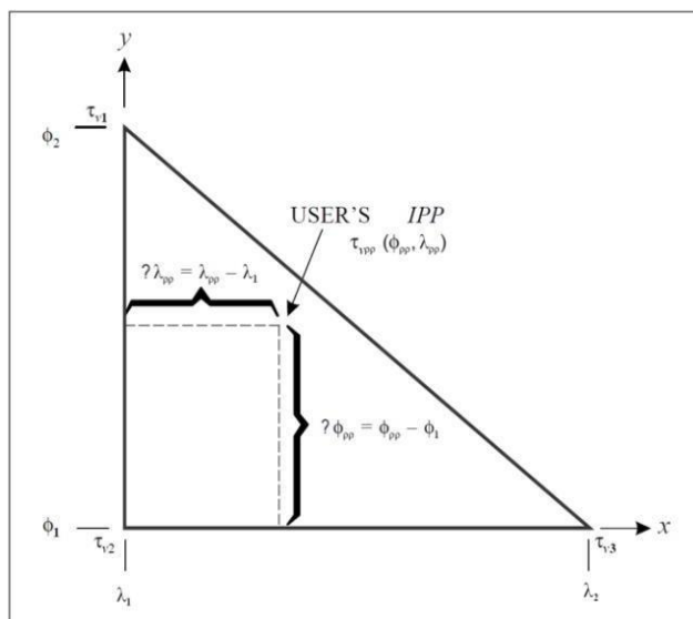
Figure B-13. IGP numbering convention (four IGPs)
