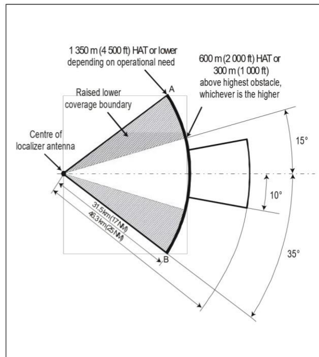
Figure C-7B. Reduced localizer coverage with respect to azimuth
