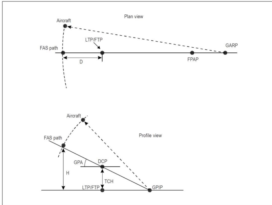
Figure D-16. FAS path definition for approaches not aligned with the runway
