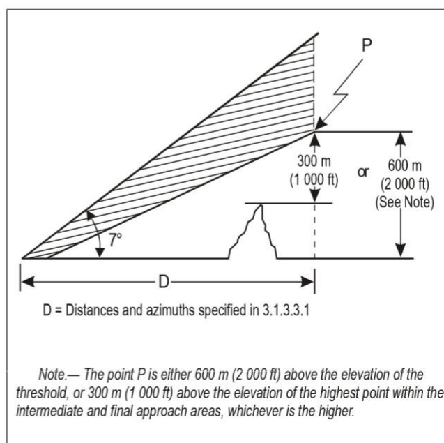
Figure C-8A. Localizer coverage with respect to elevation
