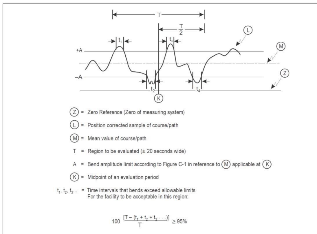
Figure C-2. Evaluation of course/path bends amplitude
