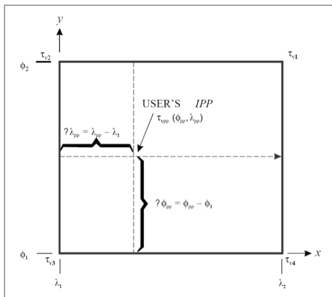
Figure B-12. Data block format
