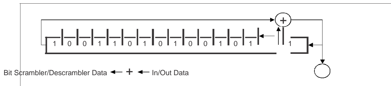
Figure D-6. Bit scrambler/descrambler
