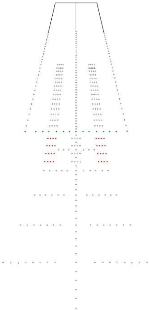
Figure 16-2. Approach and runway lighting, reduced pattern
