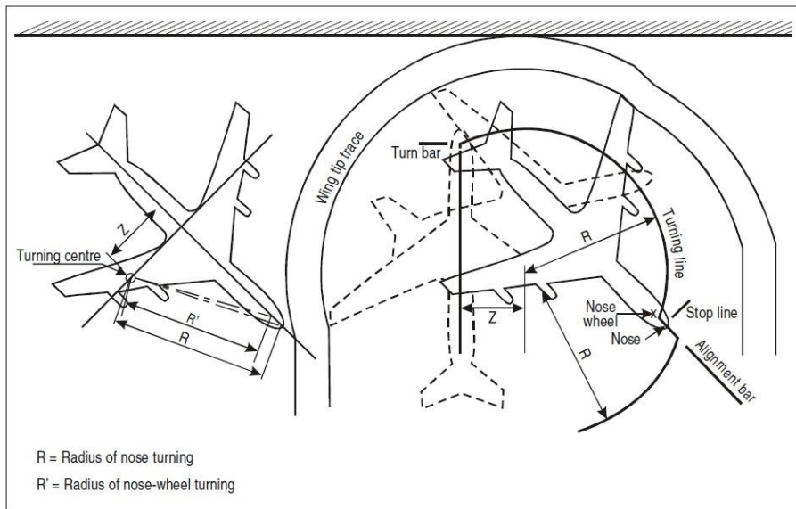
Figure 2-5. Turning line and reference bars
