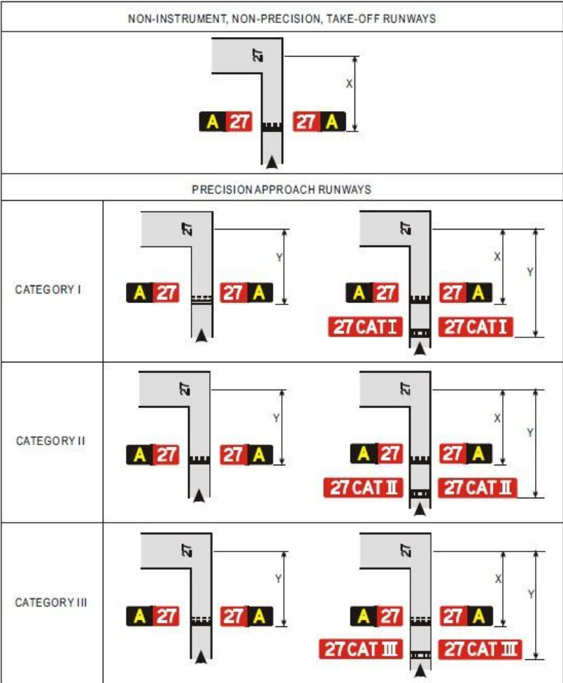
Figure 11-3. Examples of sign positions at taxiway/runway intersections
