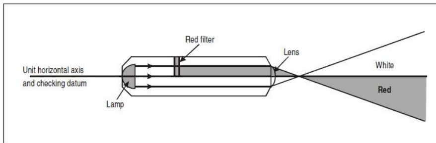
Figure 8-9. PAPI light unit
