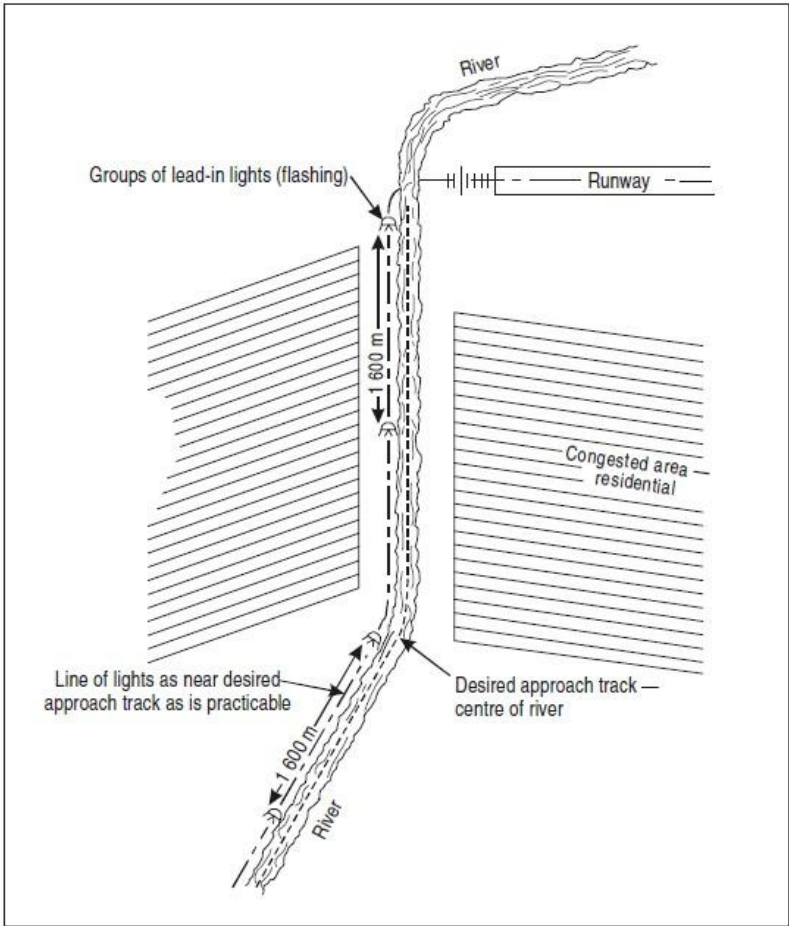
Figure 6-1. Typical layout for runway lead-in lighting system
