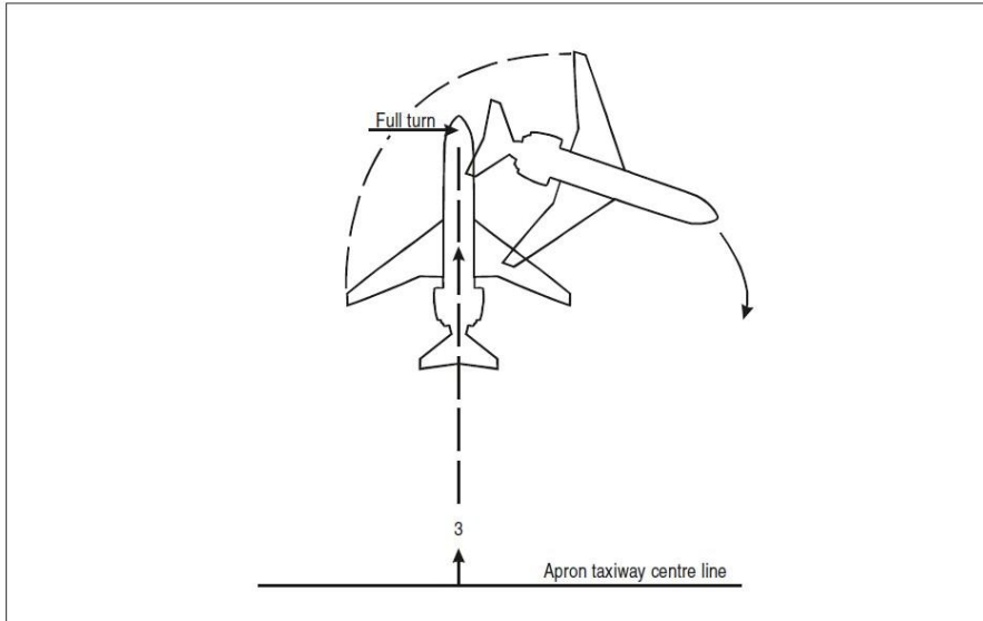
Figure 2-4. Straight lead-in line
