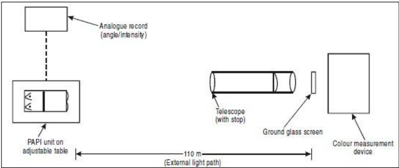
Note.— Intensity measurements were made by replacing the ground glass screen and tintometer with a small integrating sphere and photocell. Figure 8-10. Layout of test laboratory
