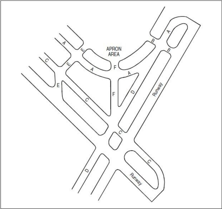
Figure 11-6. Assignment of letters to taxiways
