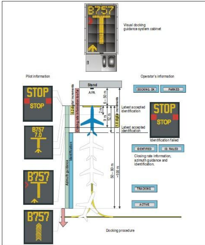
Figure 12-1. A visual docking guidance system using a graphical display and laser-based sensors to provide azimuth guidance, distance-to-go and stopping position information
