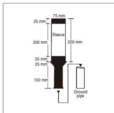
Figure 2-10. Taxiway edge marker
