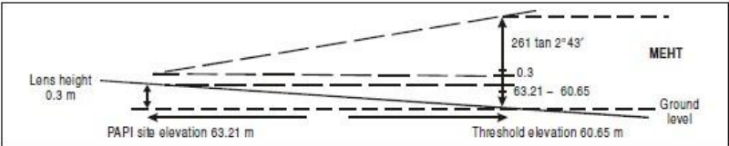
Figure 8-13. MEHT back-check
