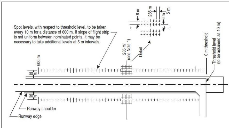
Figure 8-1. T-VASIS location survey
