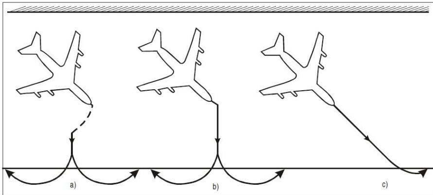
Figure 2-7. Offset nose-wheel lead-out lines
