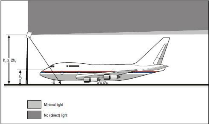
Figure 13-6. Mounting height to avoid glare
