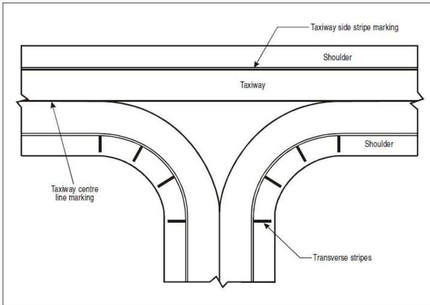
Figure 2-1. Marking of paved taxiway shoulders
