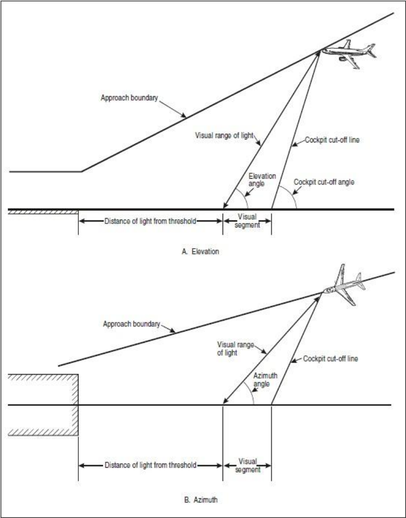
Figure 4-1. Visual segment geometry
