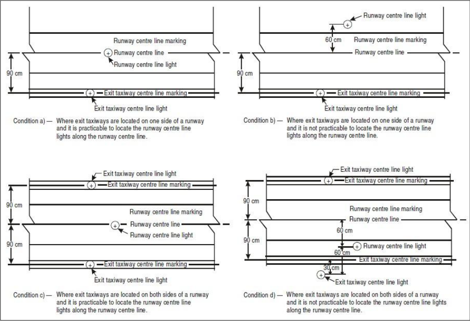
Figure 9-2. Marking and lighting of runway/taxiway intersections
