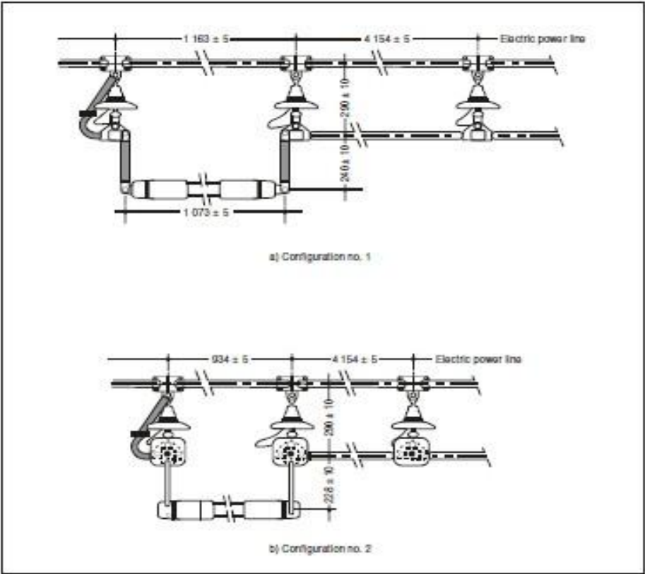
Figure 14-5. Installation of obstacle lights on high-tension wire
