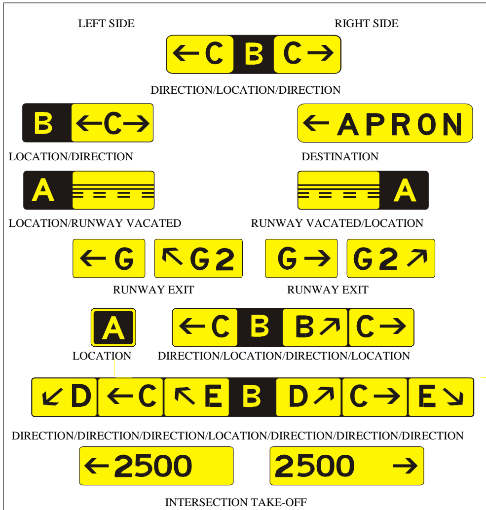
Figure 11-5. Information signs
