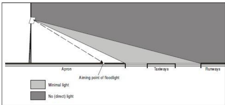
Figure 13-5. Aiming to avoid glare
