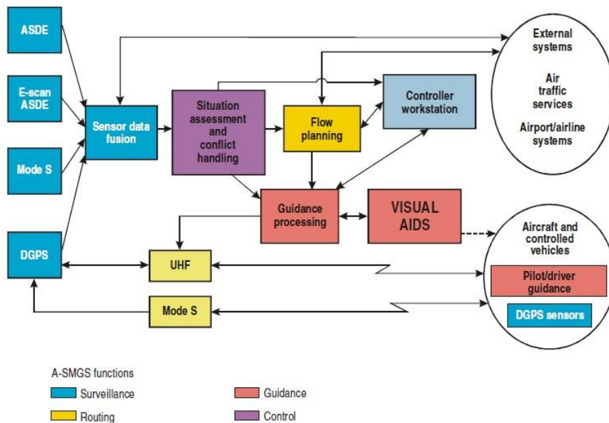
Figure 10-1. An example of A-SMGCS system architecture
