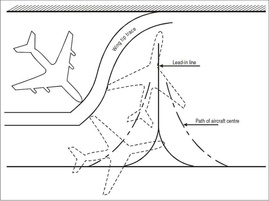
Figure 2-2. Simple nose-wheel lead-in line
