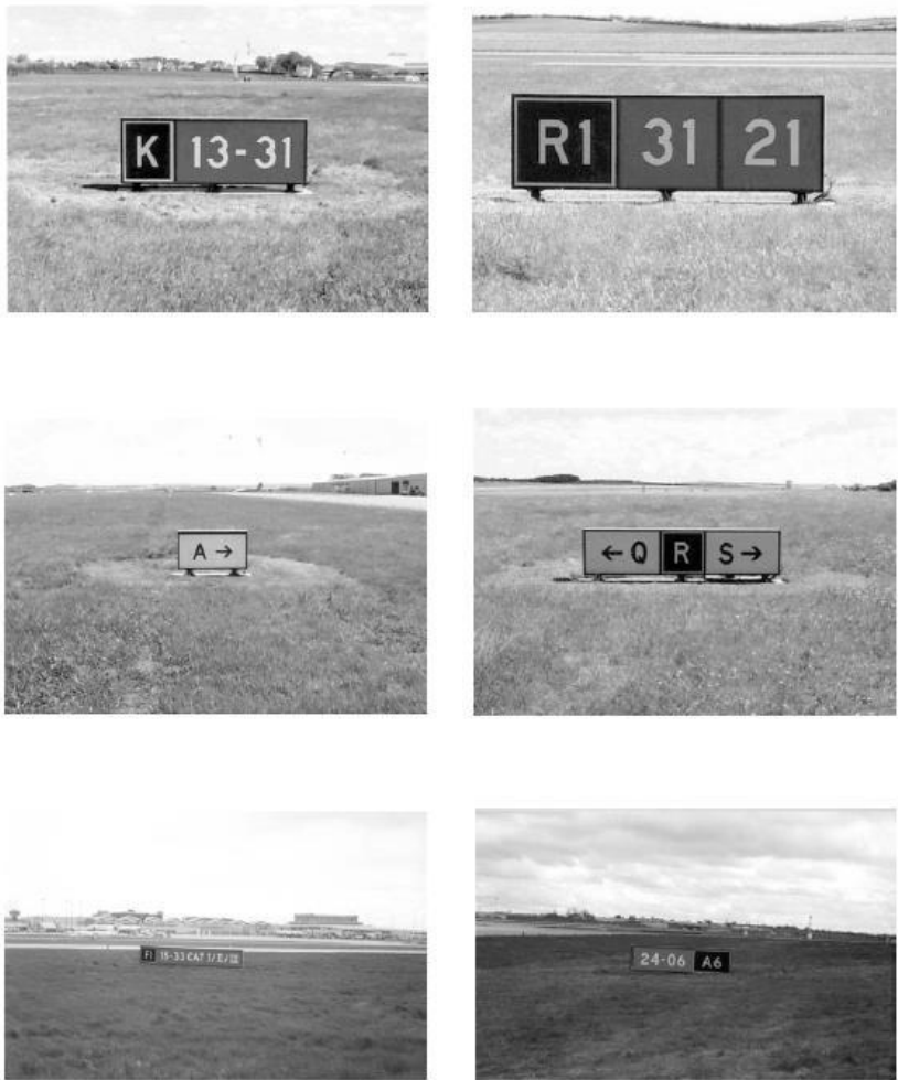
Figure 11-7. Examples of typical sign designs
