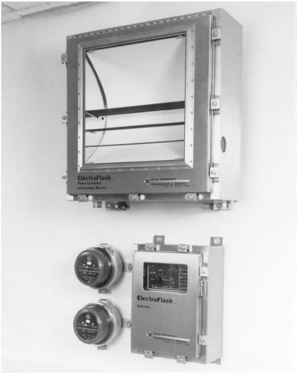
Figure 14-3. A typical high-intensity obstacle light unit
