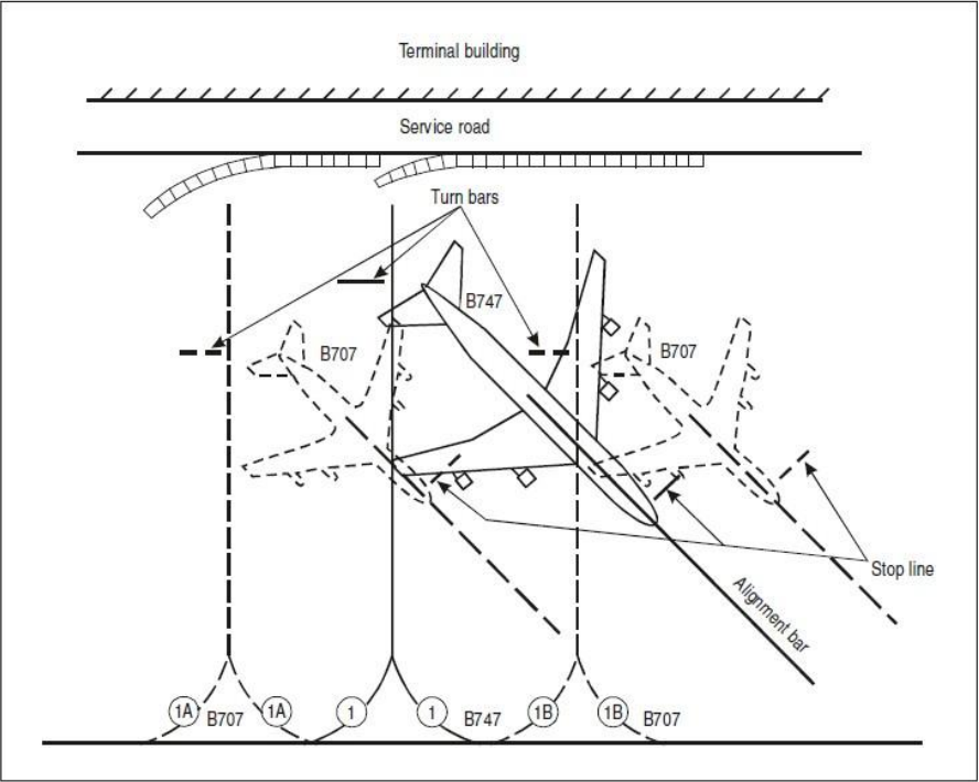
Figure 2-8. One method of marking superimposed stands
