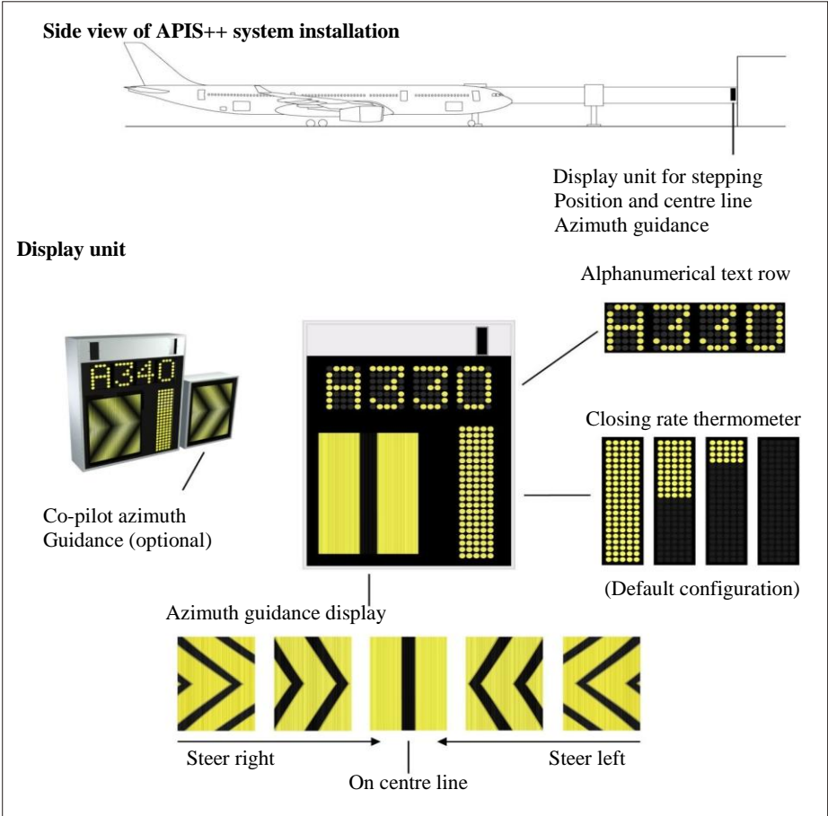
Figure 12-2. A visual docking guidance system using a graphical display (Moiré technique) to provide azimuth guidance and a laser radar to provide distance-to-go and stopping position information
