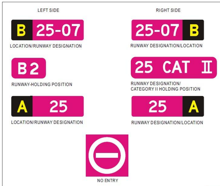
Figure 11-2. Mandatory instruction signs
