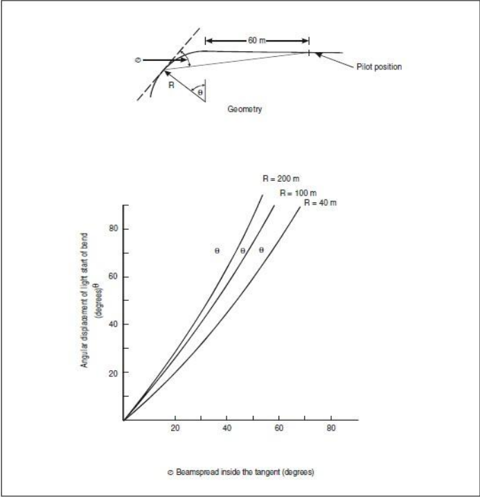
Figure 4-2. Taxiway lighting geometry
