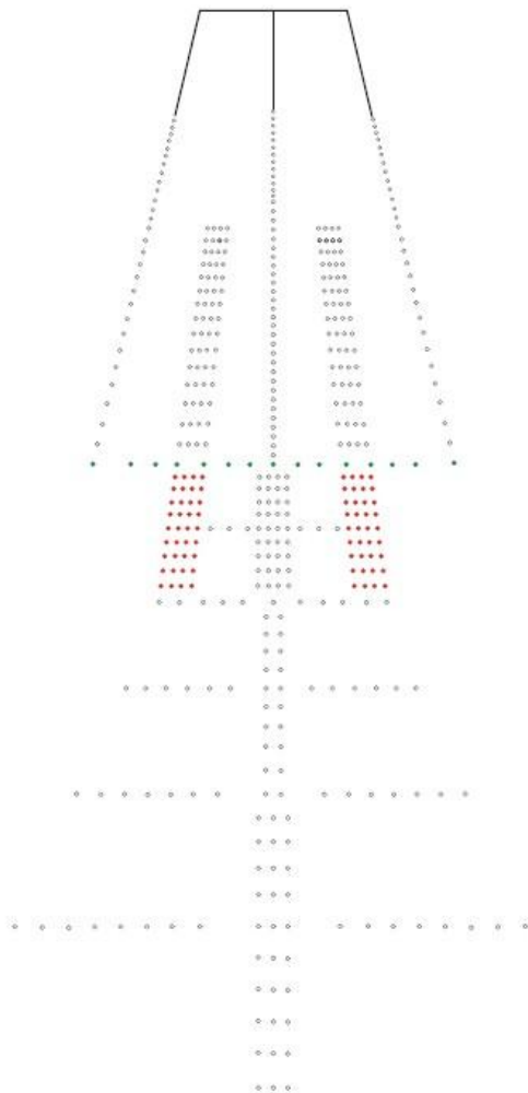
Figure 16-1. Approach and runway lighting, full pattern
