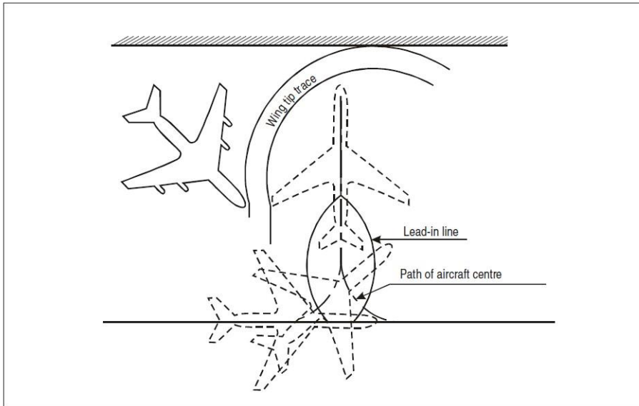
Figure 2-3. Offset nose-wheel lead-in line
