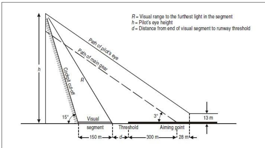
Figure A4-1. Geometry during final approach
