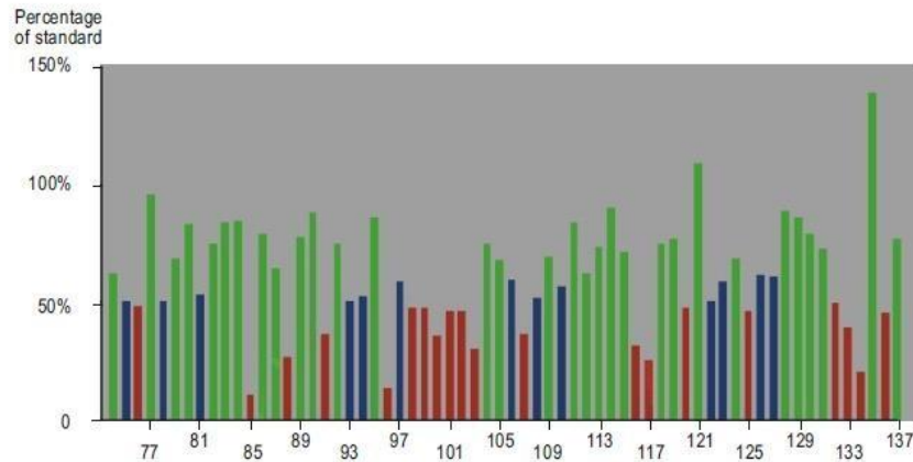
Figure 17-1. A Category III runway before differential maintenance
