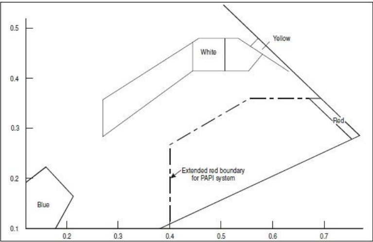
Figure 8-11. Suggested practical boundary for red PAPI
