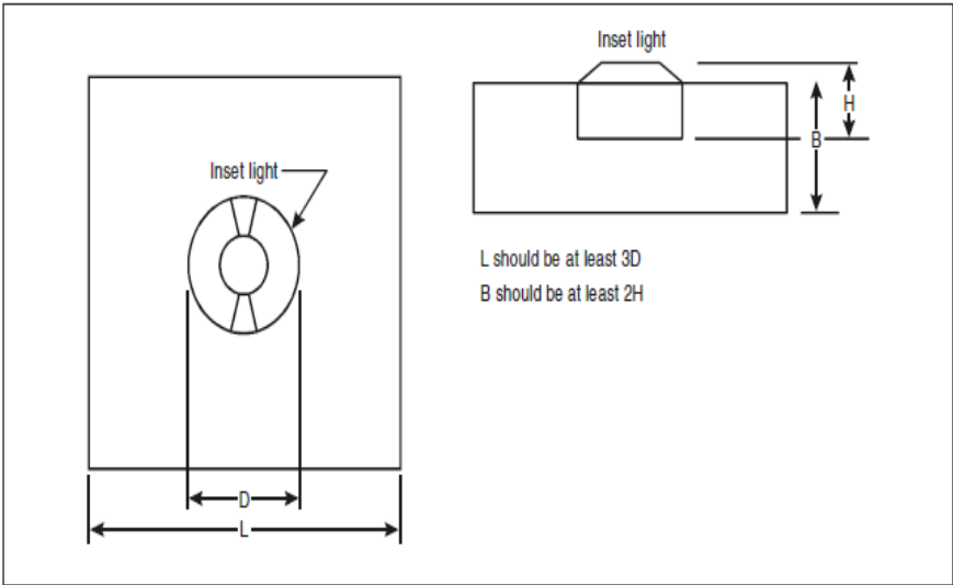
Figure 9-1. A typical container used for the temperature measurement of inset lights
