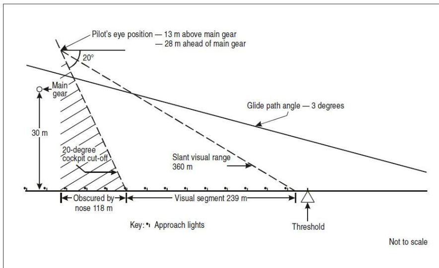
Figure 1-2. Visual segment from a large-bodied jet aircraft
