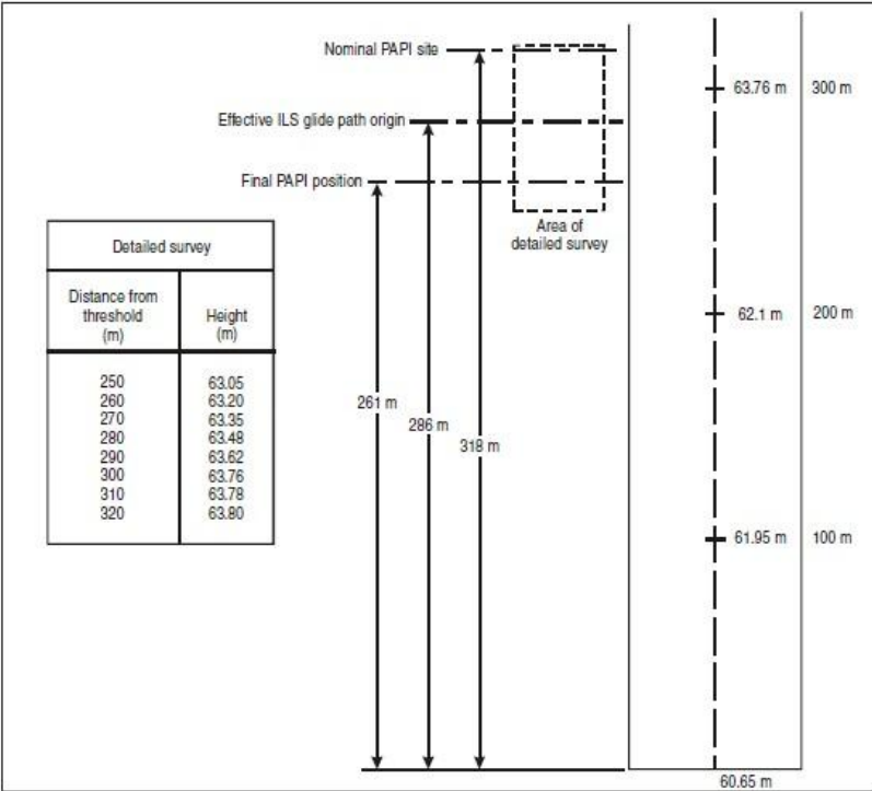
Figure 8-12. Survey data
