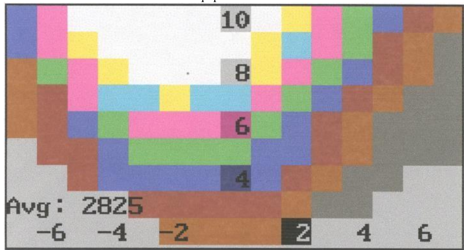
Figure 17-3A. Data from a light that is misaligned
