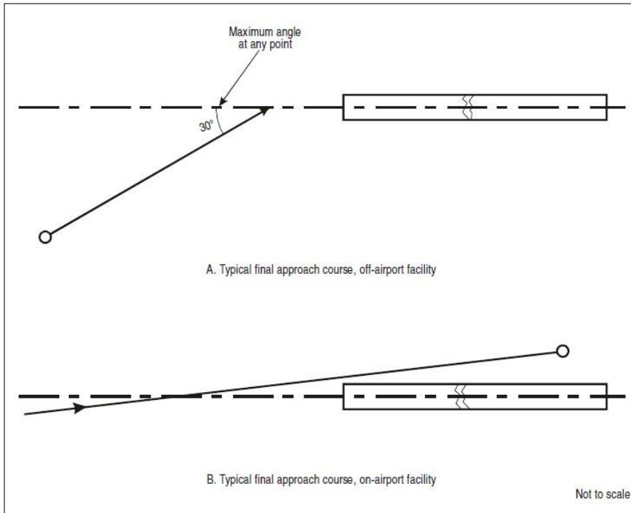
Figure 1-5. Examples of straight-in landings, non-precision aids
