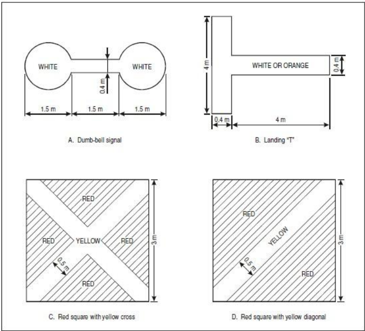
Figure 3-1. Signal panels and landing “T”
