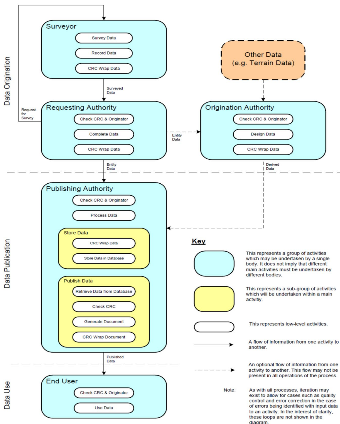
Figure 2: Aeronautical Data Process Diagram
