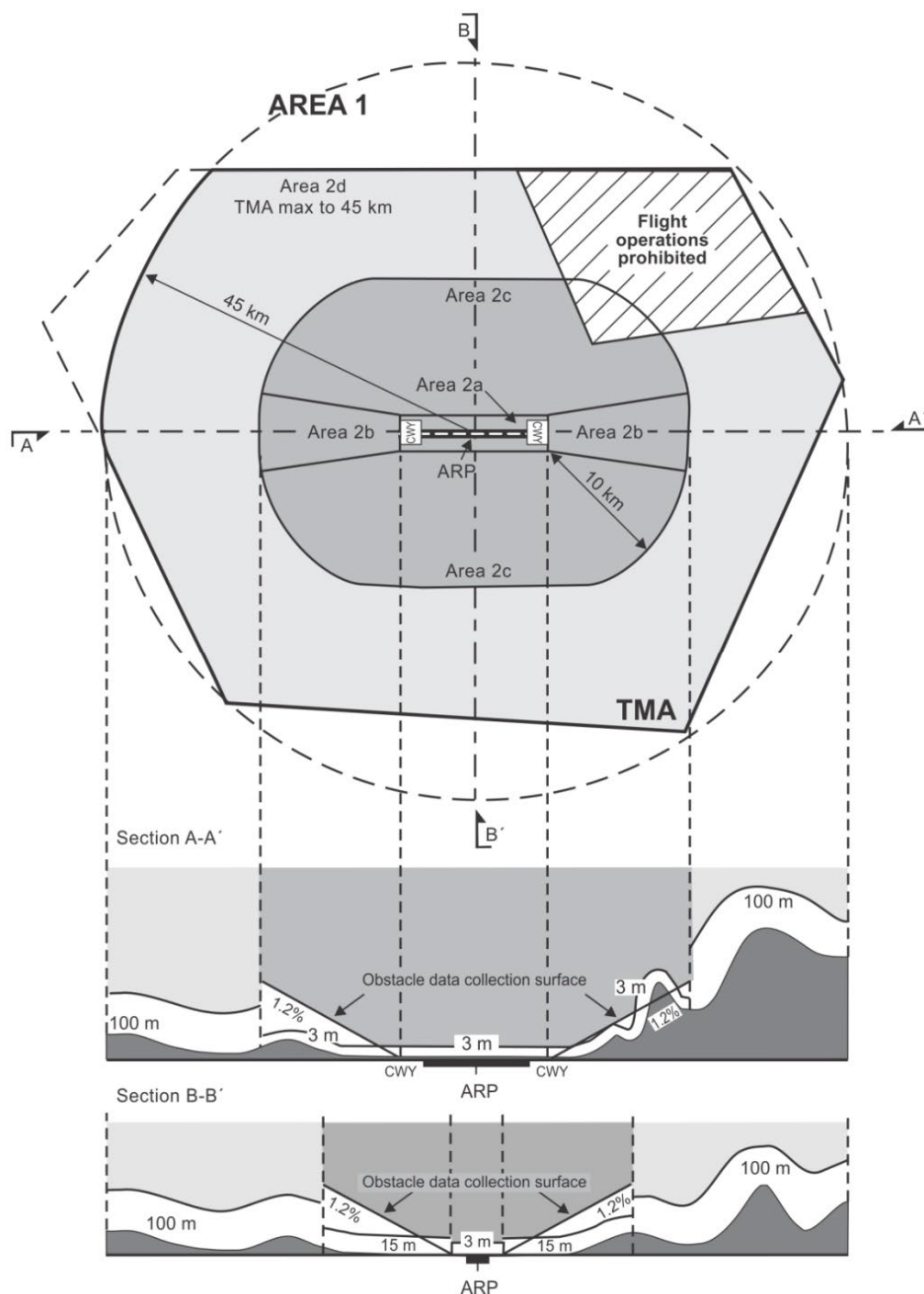
Figure 8: Obstacle data collection surfaces – Area 1 and Area 2
