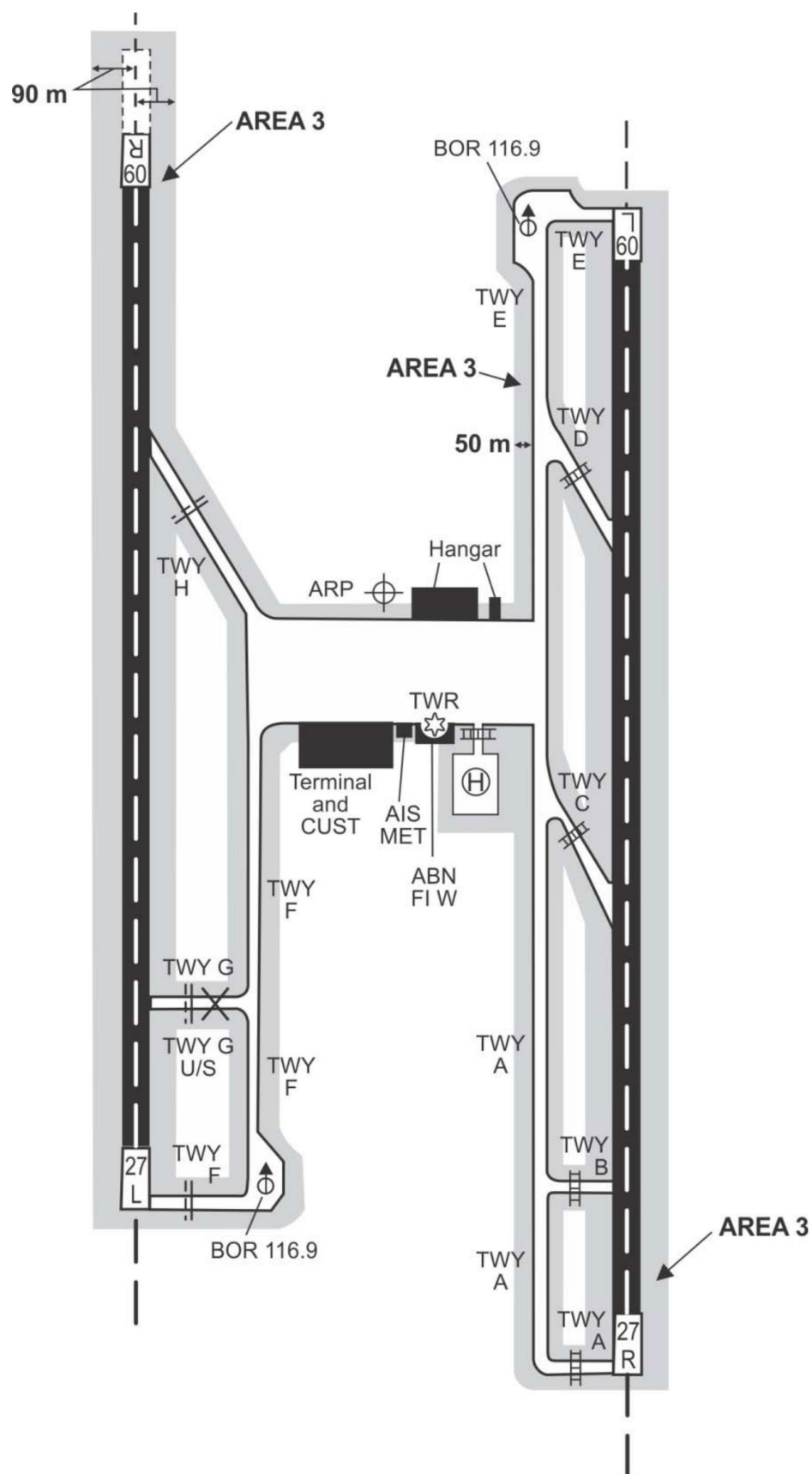
Figure 9: Terrain and obstacle data collection surface – Area 3
