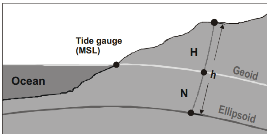
Figure 6: Geoid as Reference Surface for Heights
