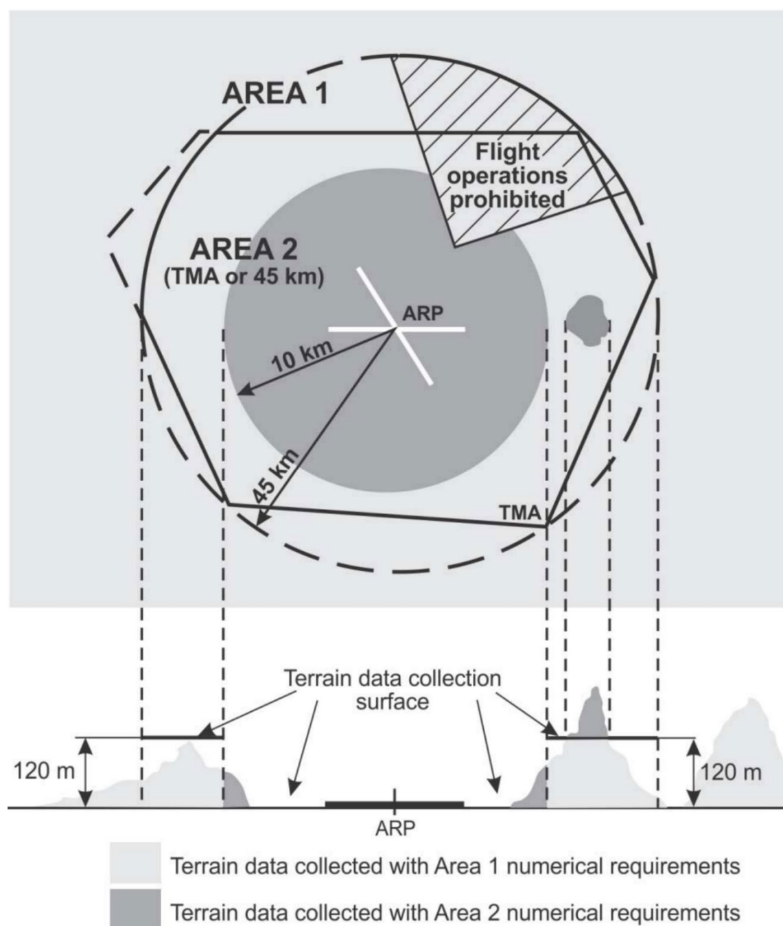
Figure 7: Terrain data collection surfaces - Area 1 and Area 2
