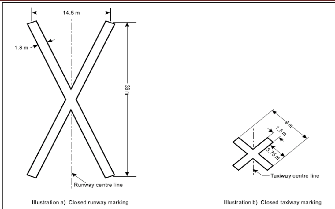
Figure 7-1. Closed runway and taxiway markings
