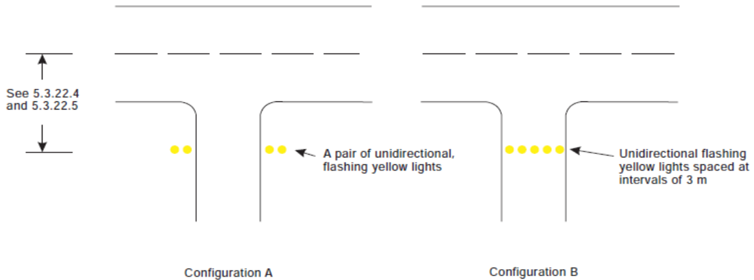
Figure 5-29. Runway guard lights
