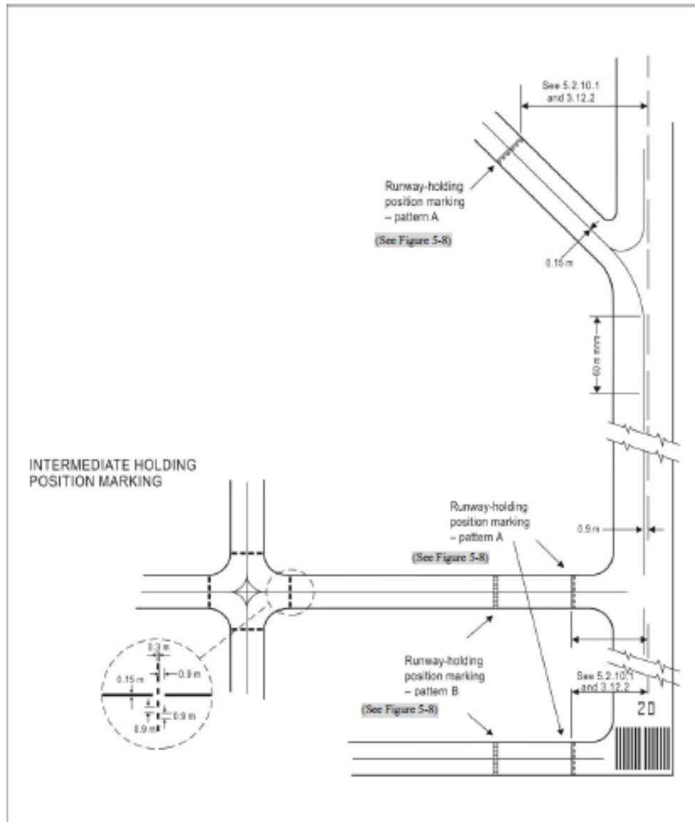
Figure 5-6. Taxiway markings
