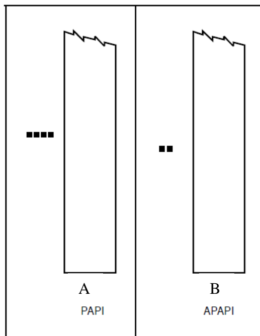
Fig 5-16 Visual approach slope indicator systems
