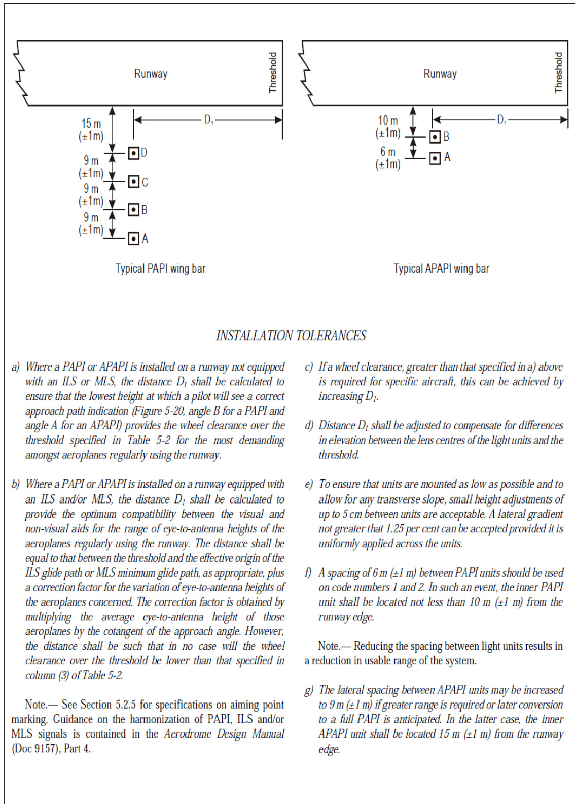
Figure 5-19. Siting of PAPI and APAPI
