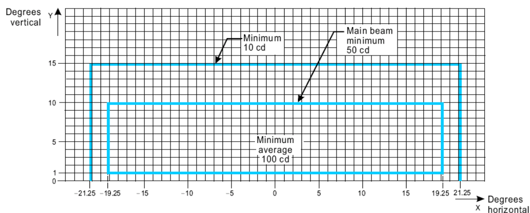
Figure A2-13. Isocandela diagram for taxiway centre line (7.5 m spacing), no-entry and stop bar lights in straight sections intended for use in runway visual range conditions of less than a value of 350 m
